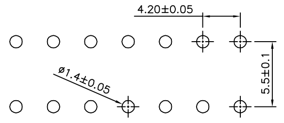
Recommended P.C.B. Layout PCB Thickness:1.6mm
